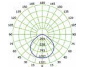
The average illuminance effective figure
