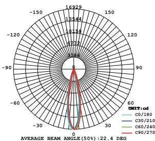
LUMINOUS INTENSITY DISTRIBUTION
