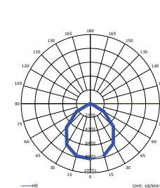
LUMINOUS INTENSITY DISTRIBUTION DIAGRAM
