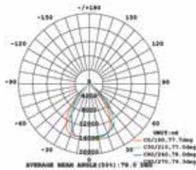
INHOUS INTENSITY DISTRIBUTION DIAGRAM
